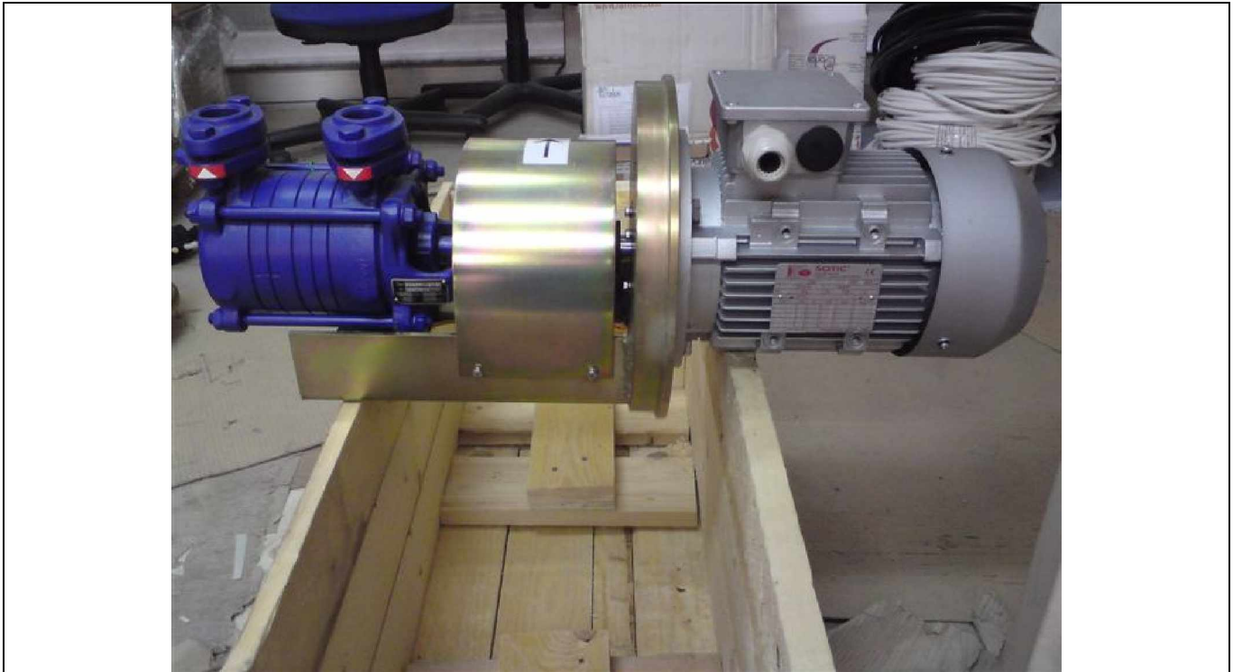
Figure 3: Brand New MK-III Motor – Sampling Pump Assembly in full compliance with MEPC108 (49).
